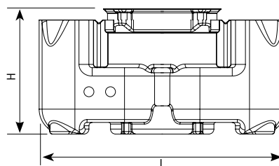
DN 200 / DN 300
